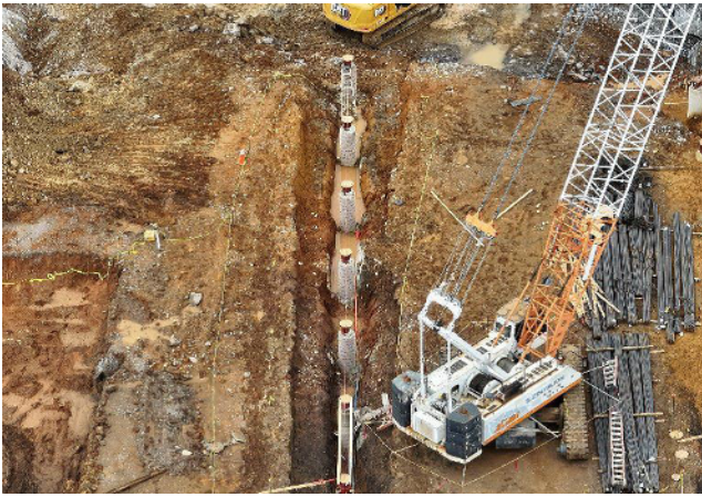
Aerial View of Pier Installation
